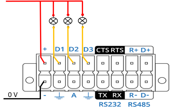
Fig. 7 Connecting D1, D2 and D3 as outputs
