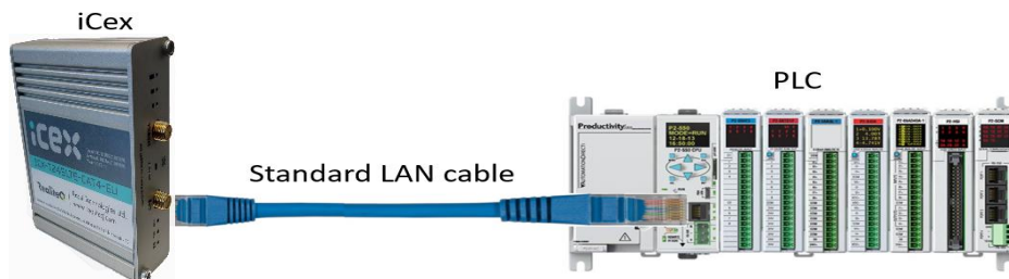
Fig. 1 Connect direct iCex to device (PLC) via Ethernet
