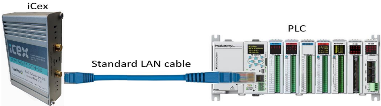
Fig. 11 Connecting third party I/O card to iCex via Modbus RTU/TCP converter
