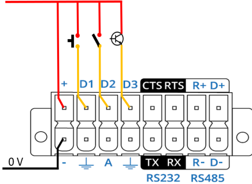
Fig. 6 Connecting D1, D2 and D3 as inputs
