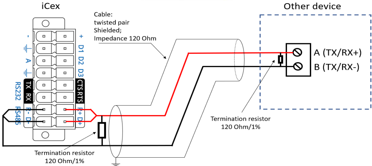
Fig. 5 RS485 2-wire connection to one device
